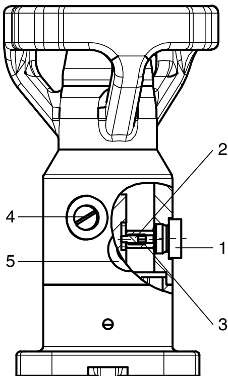
Setting the damping cam
