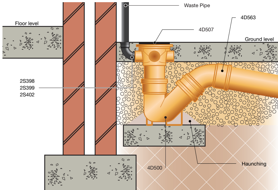
Figure 12: Typical waste connection to Sealed Hopper
