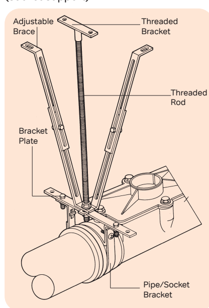
Figure 39: Suspended Bracketing (socket support)
