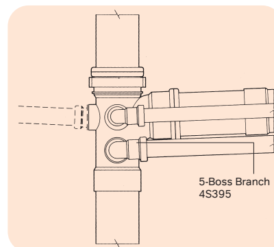
Figure 50: Connection of multiple wastes
