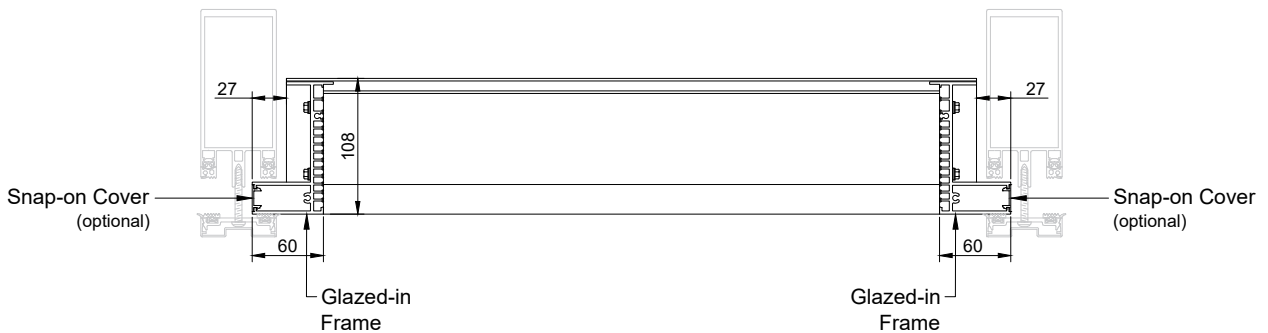
PLAN VIEW (1:6 @A4)
