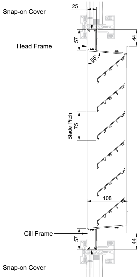
SECTION ON ELEVATION (1:6 @A4)
