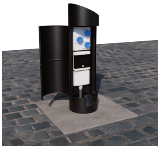
325mm unit open
