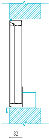
Section on elevation
