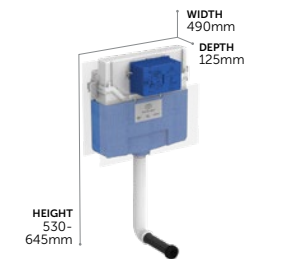
120 Depth WC Concealed Cistern
