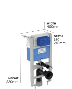
820mm Wall Hung WC Frame
