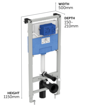
1150mm Wall Hung WC Frame
