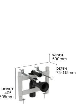
Half Frame for Wall Hung Pans
