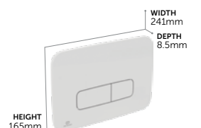
Oleas M3 Mechanical Dual Flushplate
