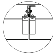
Hidden mullion at a joint between blade lengths
