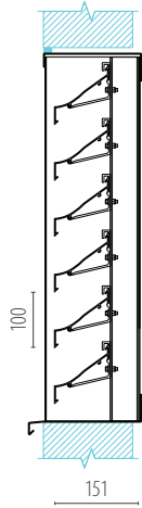
Section on elevation
