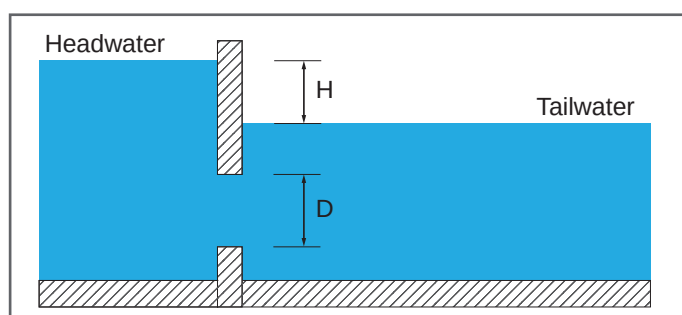
Figure 3(b) - Submerged flow.
